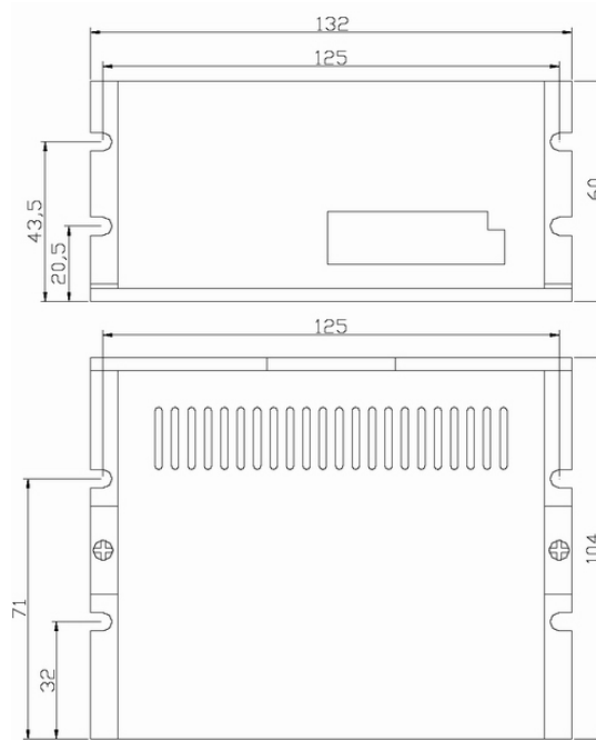
Figure 1: Mechanical specifications
